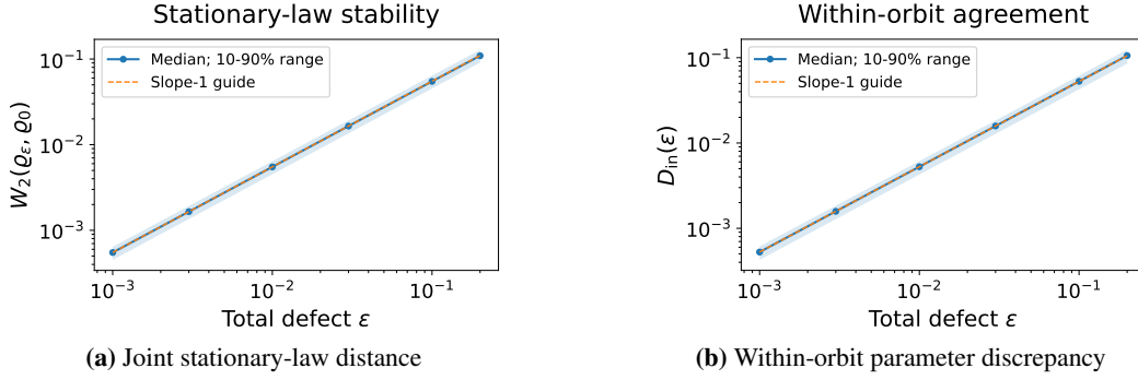
Figure 5: Stationary perturbation responses. Solid curves and shading show medians and 10th–90th percentiles over 20 fixed directions. Dashed lines are slope-one guides, not theoretical bounds.
