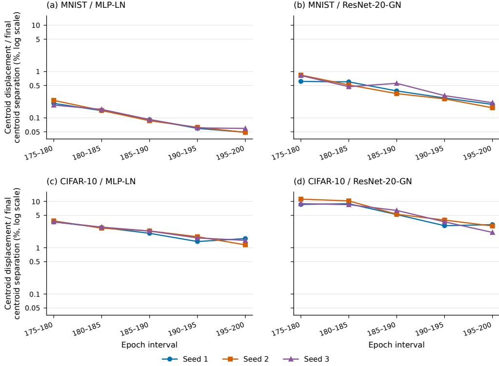
Figure 9: Main orbit-centroid motion over consecutive five-epoch intervals. Points show 100\rho(a, a + 5) for each seed, normalized by the smallest centroid separation at epoch 200. The vertical axis is logarithmic.
