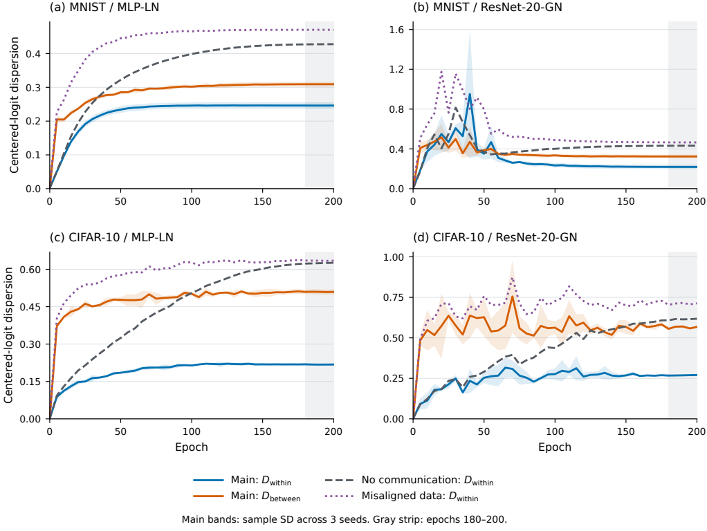
Figure 8: Prediction-space dispersion during training. Curves show three-seed means; bands indicate \pm one sample SD for Main. The gray strip marks epochs 180–200. Vertical scales vary across panels.
