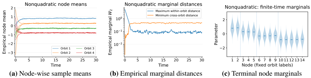
Figure 7: Nonquadratic finite-time grouping. (a) Node-wise sample means; colors denote orbits. (b) Maximum within-orbit and minimum cross-orbit empirical W_2 . (c) Terminal violin plots at T = 30 , with sample means and orbit separators. Empirical fluctuations include finite-sample error.
