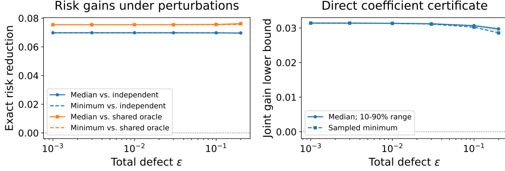
Figure 6: Stationary risk gains (left) and direct joint certificate \gamma(\theta_\varepsilon) (right). Solid curves, shading, and dashed curves show medians, 10th–90th percentiles, and sampled minima over 20 fixed directions. These summaries are not confidence bounds or worst-case guarantees.
