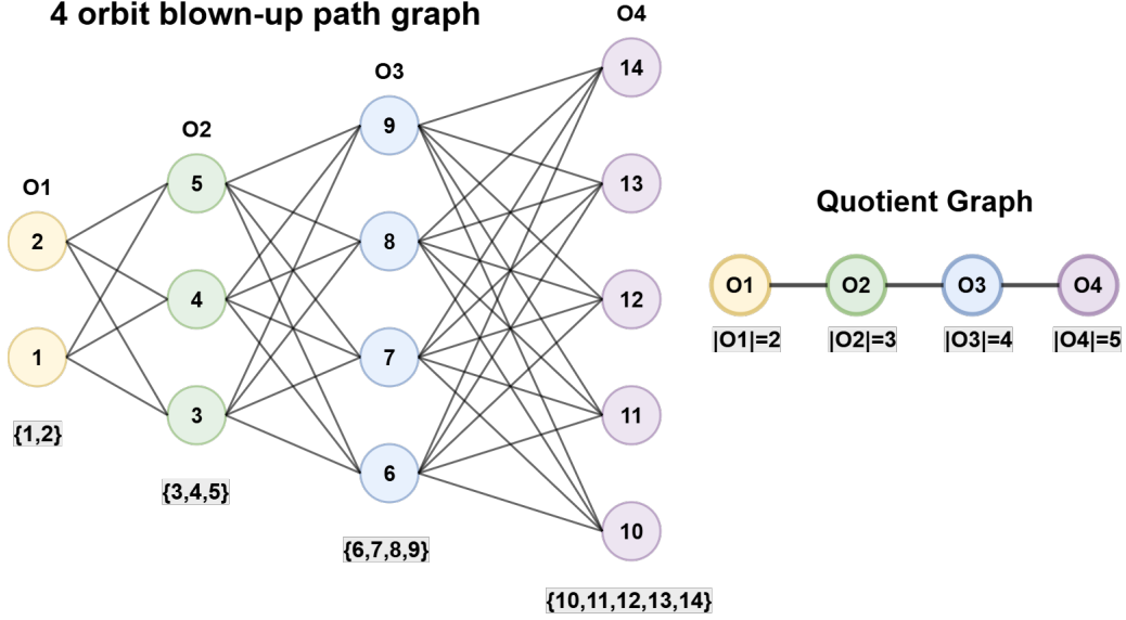
Figure 3: Four-orbit blown-up path graph and its quotient graph. Colors indicate automorphism orbits.
