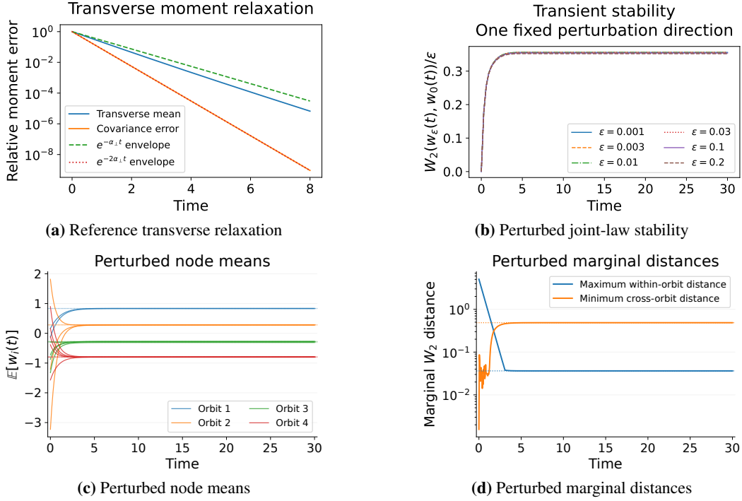
Figure 4: Temporal validation from exact affine moments. (a) Reference transverse errors and exponential bounds. (b) Joint-law W_2/\varepsilon for seed 101 at six defect levels. (c)–(d) Perturbed means and marginal distances ( \varepsilon = 0.1 , seed 101); dotted lines are stationary limits. Same-orbit means share a color.
