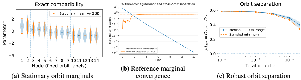
Figure 1: Orbit structure and robustness. (a) Reference marginals with stationary means and \pm 2 standard deviations. (b) Marginal W_2 under exact compatibility: within-orbit maximum and cross-orbit minimum. (c) Separation margins under joint perturbations: median (solid), sampled minimum (dashed), and 10th–90th percentiles (shaded).
